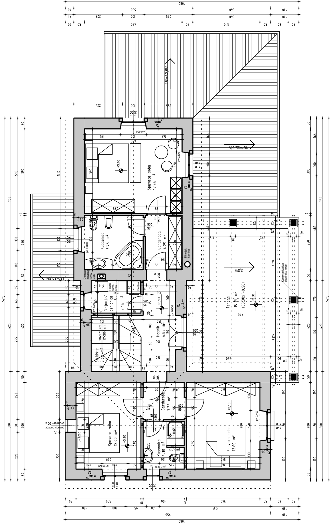
First floor Scale 1:100
